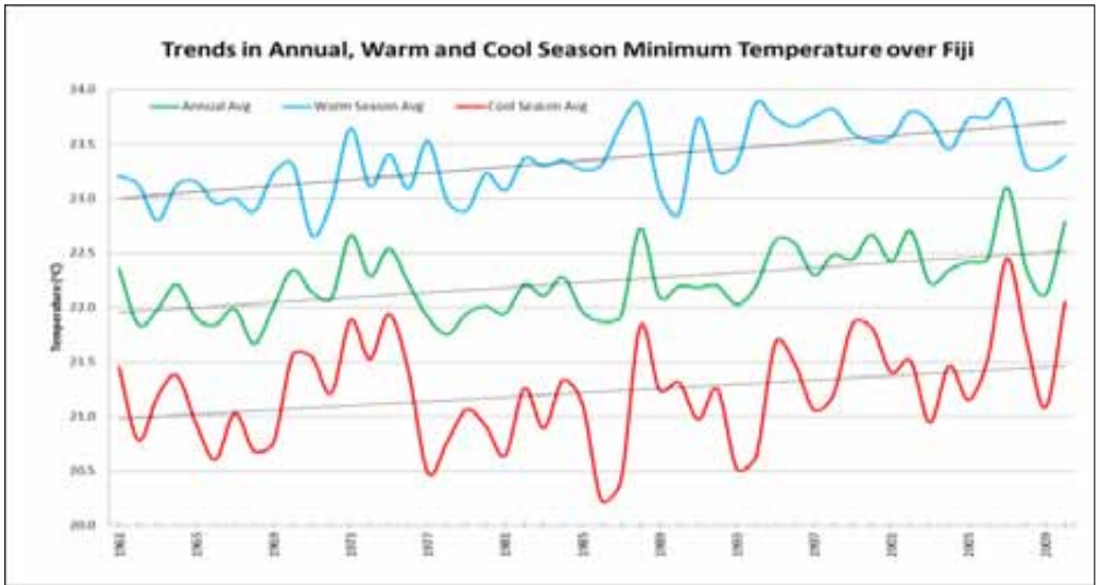
Figure A1-2: Inter-annual and seasonal variation in minimum temperature over Fiji, 1961 to 2010 Data source: Fiji Meteorological Services 2011
