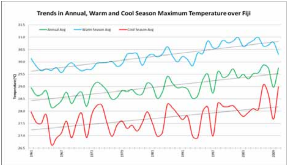
Figure A1-3: Inter-annual and seasonal variation in maximum temperature over Fiji, 1961 to 2010 Data source: Fiji Meteorological Services 2011
